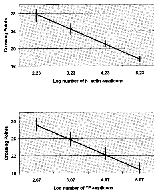
Fig. 1. Reproducibility of the calibration curves for \beta -actin (top: n = 57 ) and TF (bottom: n = 14 ).
