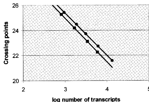
Fig. 2. PCR amplification efficiencies of \beta -actin (●) and TF (■).
